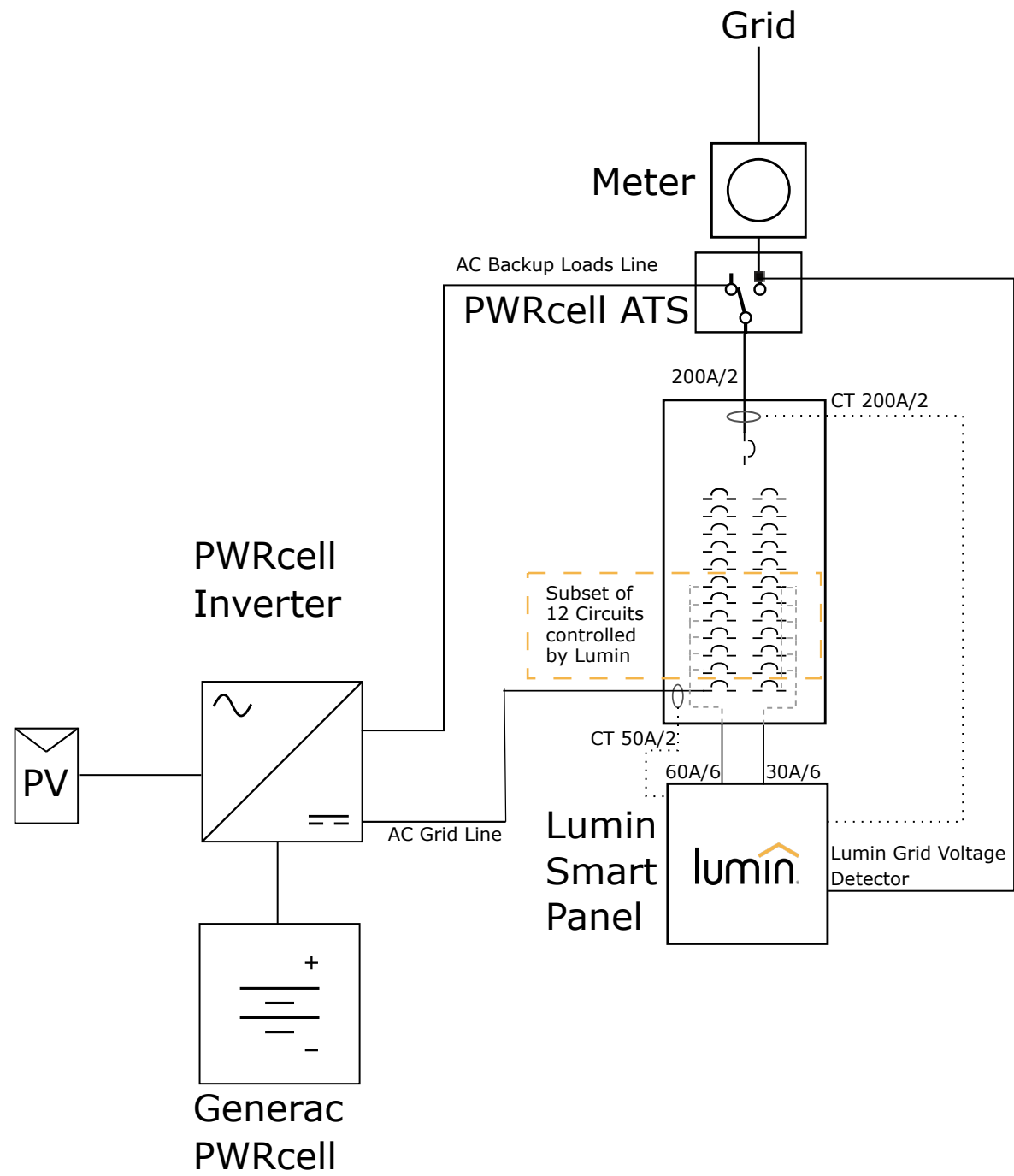
Single Line Diagram Lumin Smart Panel with Generac PWRcell ESS on Main Distribution Panel
