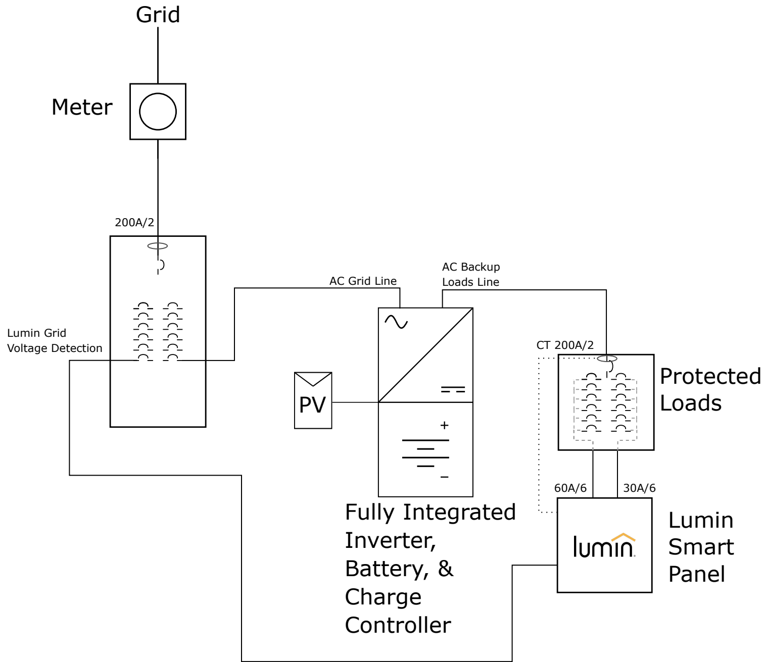
Single Line Diagram Lumin Smart Panel with DC Coupled System on Protect Loads Panel
