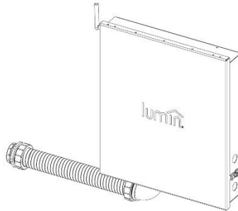
1 Outdoor LSP with Conduit, Conduit Bushings & Wire Whips Attached
